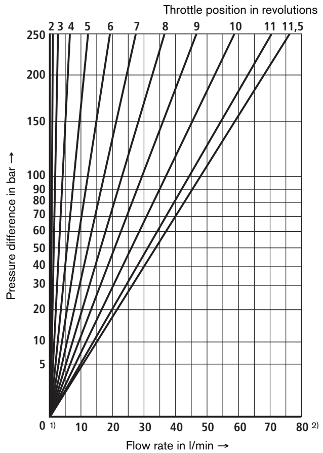
\Delta p - q_v curves for Z2FS 6...-4X/.1QXCJ
